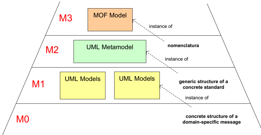
Fig. 1. Metamodel levels
